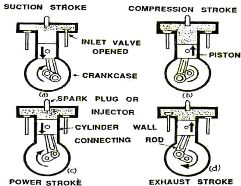
fig four stroke diesel engine
