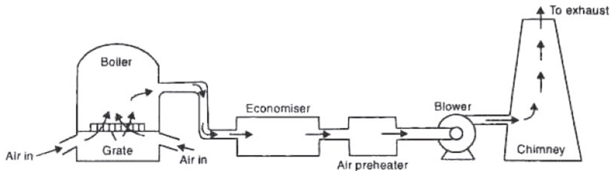
Figure: Induced fan draught
