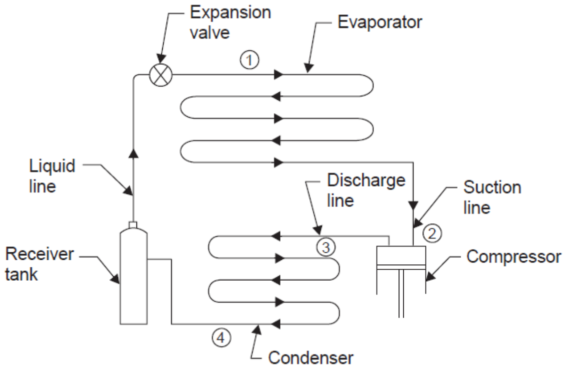
Vapour compression system.
