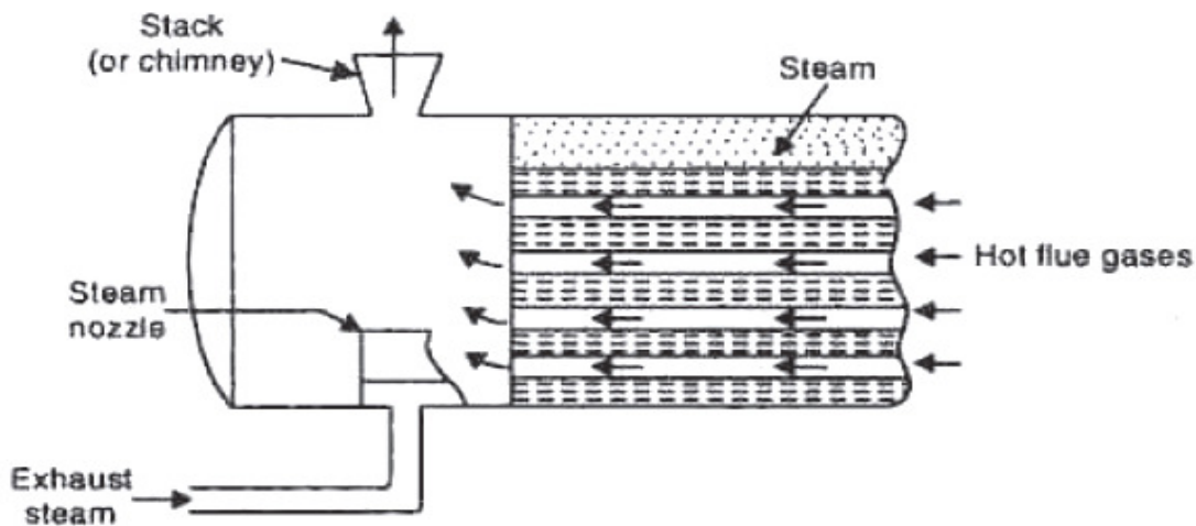
Figure: Steam Jet draught
